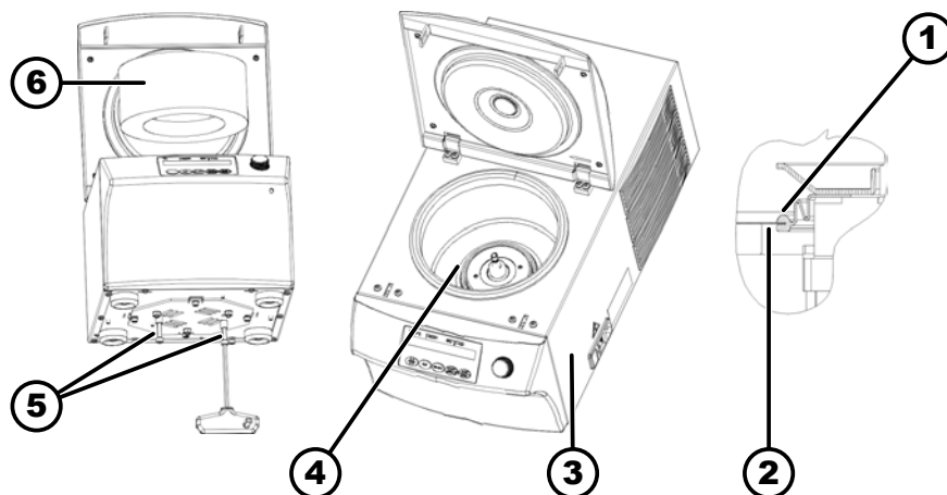
Fig. 14: Transport lock
